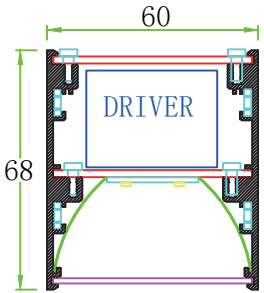
Section Detail
