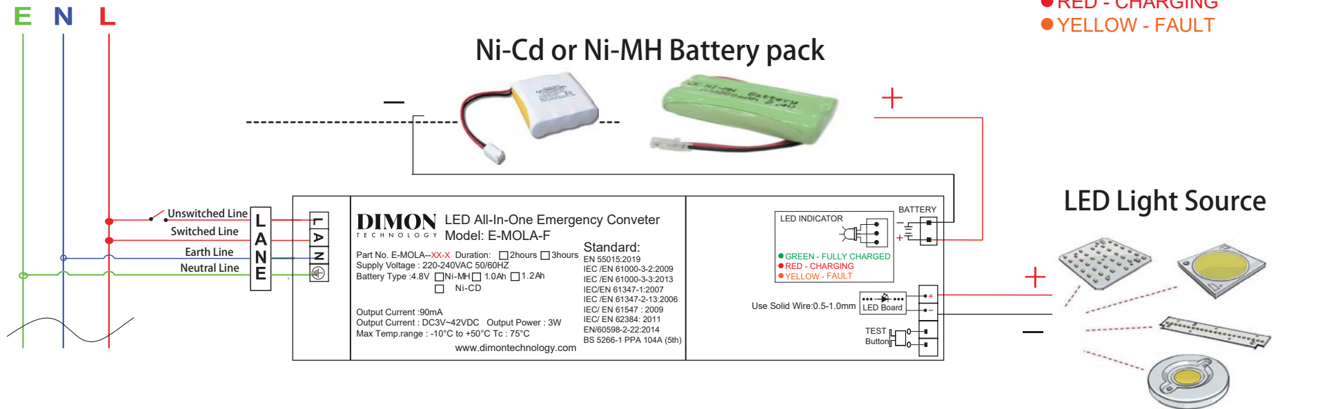
100% Output wiring with general lighting switch diagram 輸出接駁燈制開關接線圖
