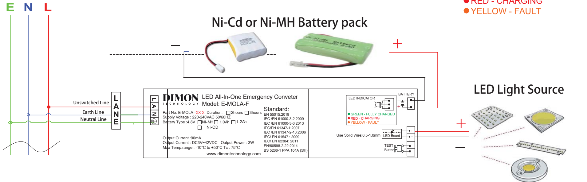
100% Output wiring (Non-Maintained Type) 輸出接線圖(後備式)
