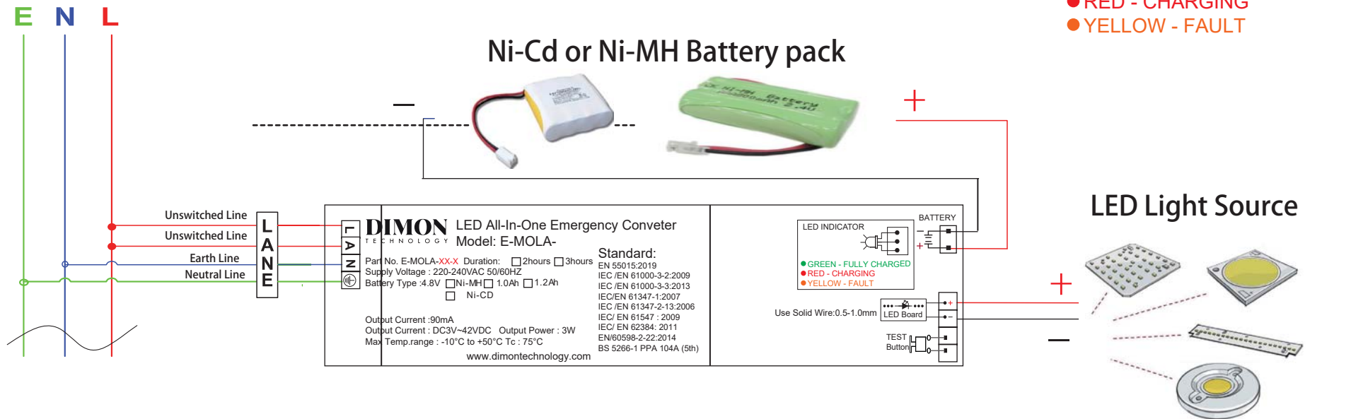
100% Output wiring (Maintained Type) 輸出接線圖(長明式)
