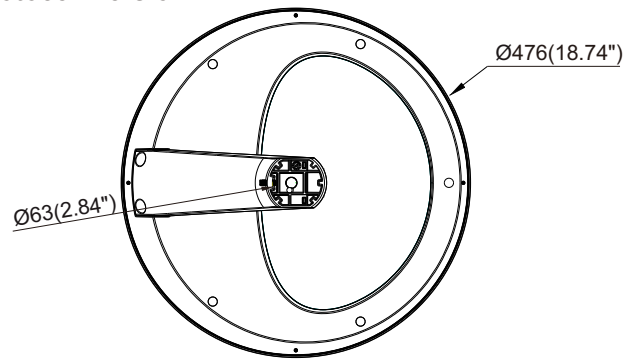
Photocell Version
