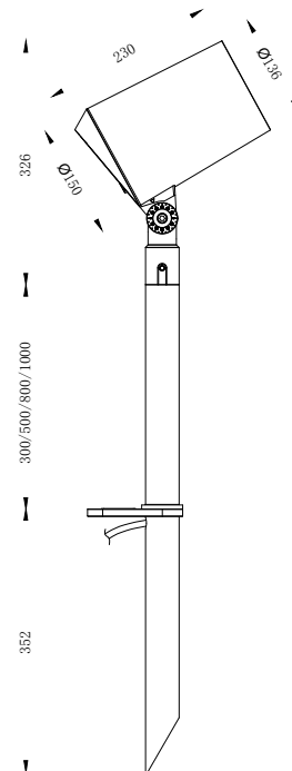
Pole & Spike Mount
