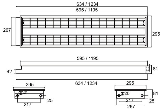
2x18W LED T8 or LED T5
