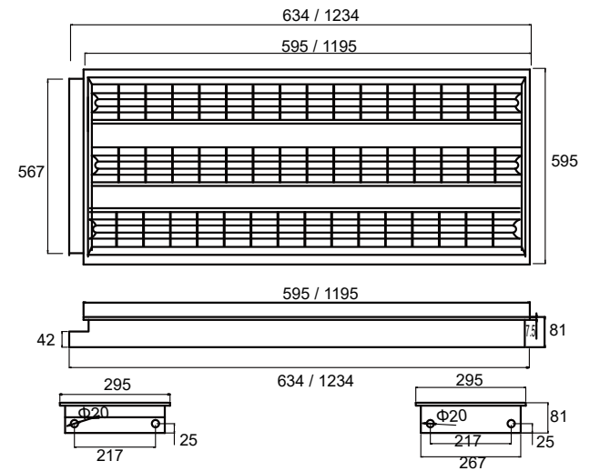
3x18W LED T8 or LED T5
