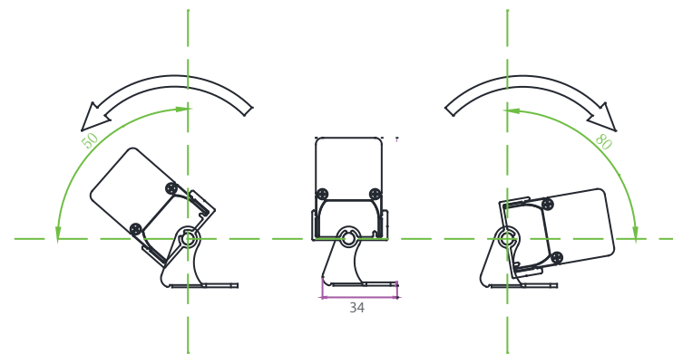
Adjustable Bracket C Rotation: +50deg / -80deg
