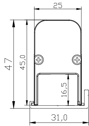
Surface Mount Bracket -B
