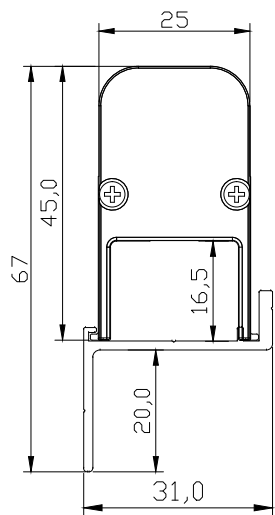
Surface Mount Bracket -A
